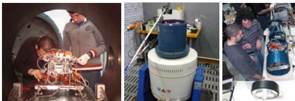
Figure 9. Vacuum chamber (left), shaker (middle), service system simulator (right).
